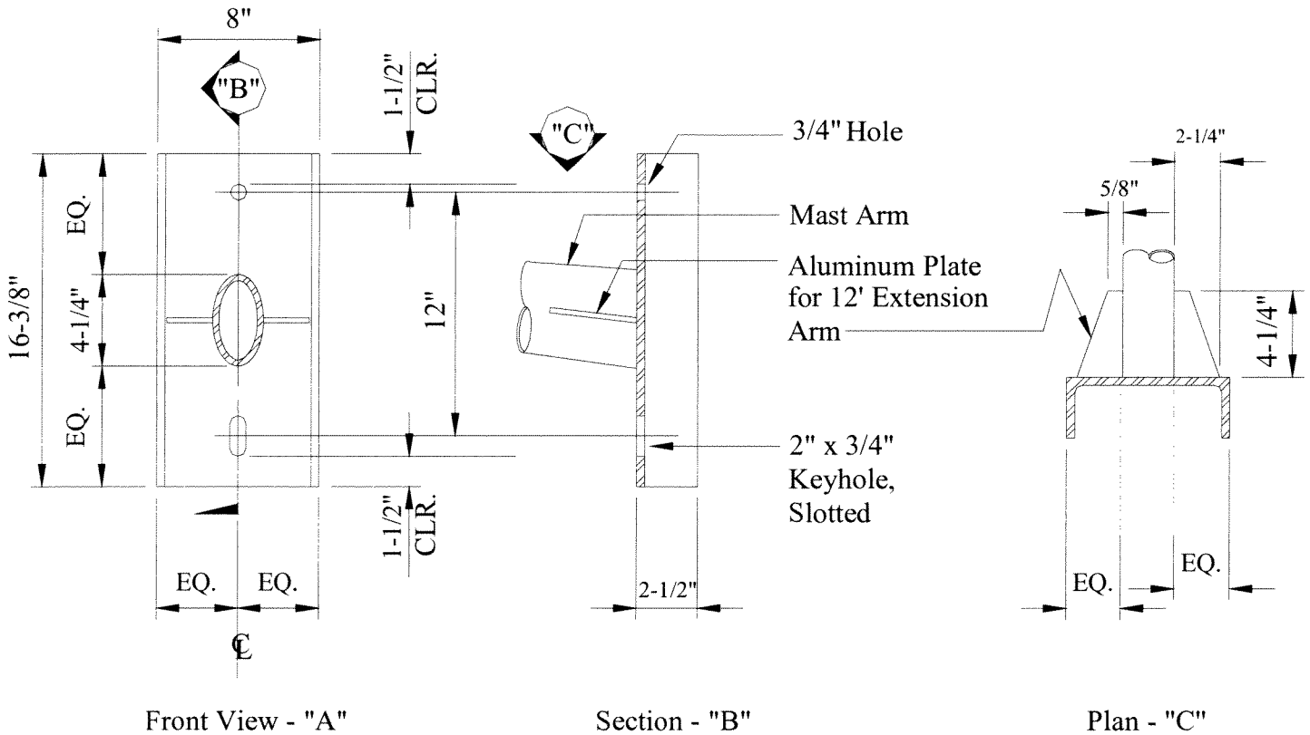
Mounting Plate Detail Figure 2
