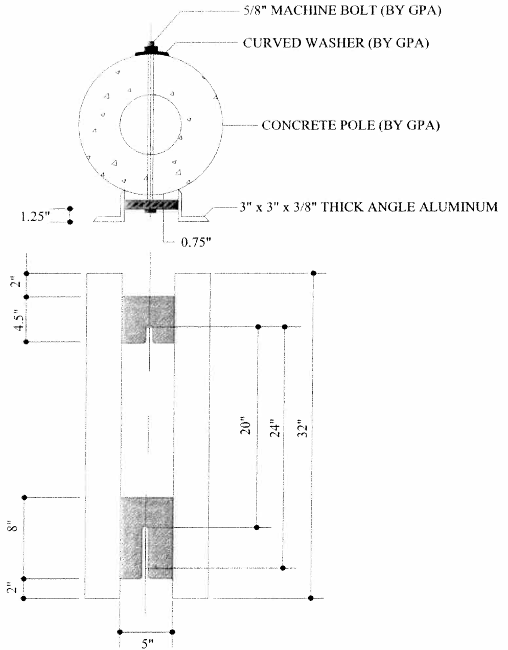
Figure A Mounting Bracket
