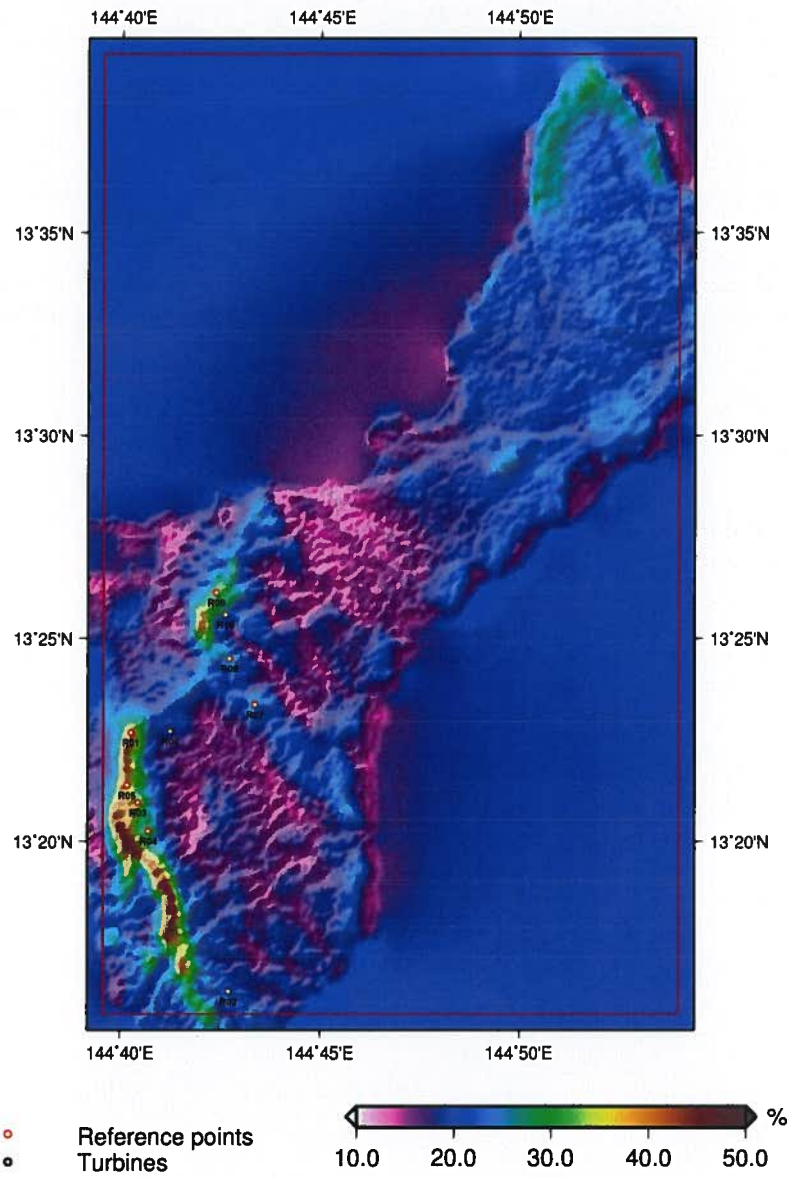
Figure 2: Mean capacity factor for the GEVMP32/275L turbine at 55m.
