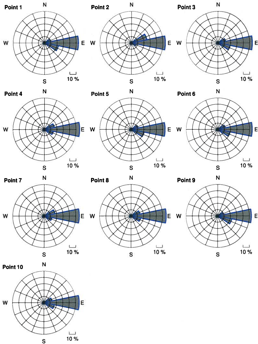
Figure 5: Annual power roses (for the GEVMP32/275L turbine) for all reference points
