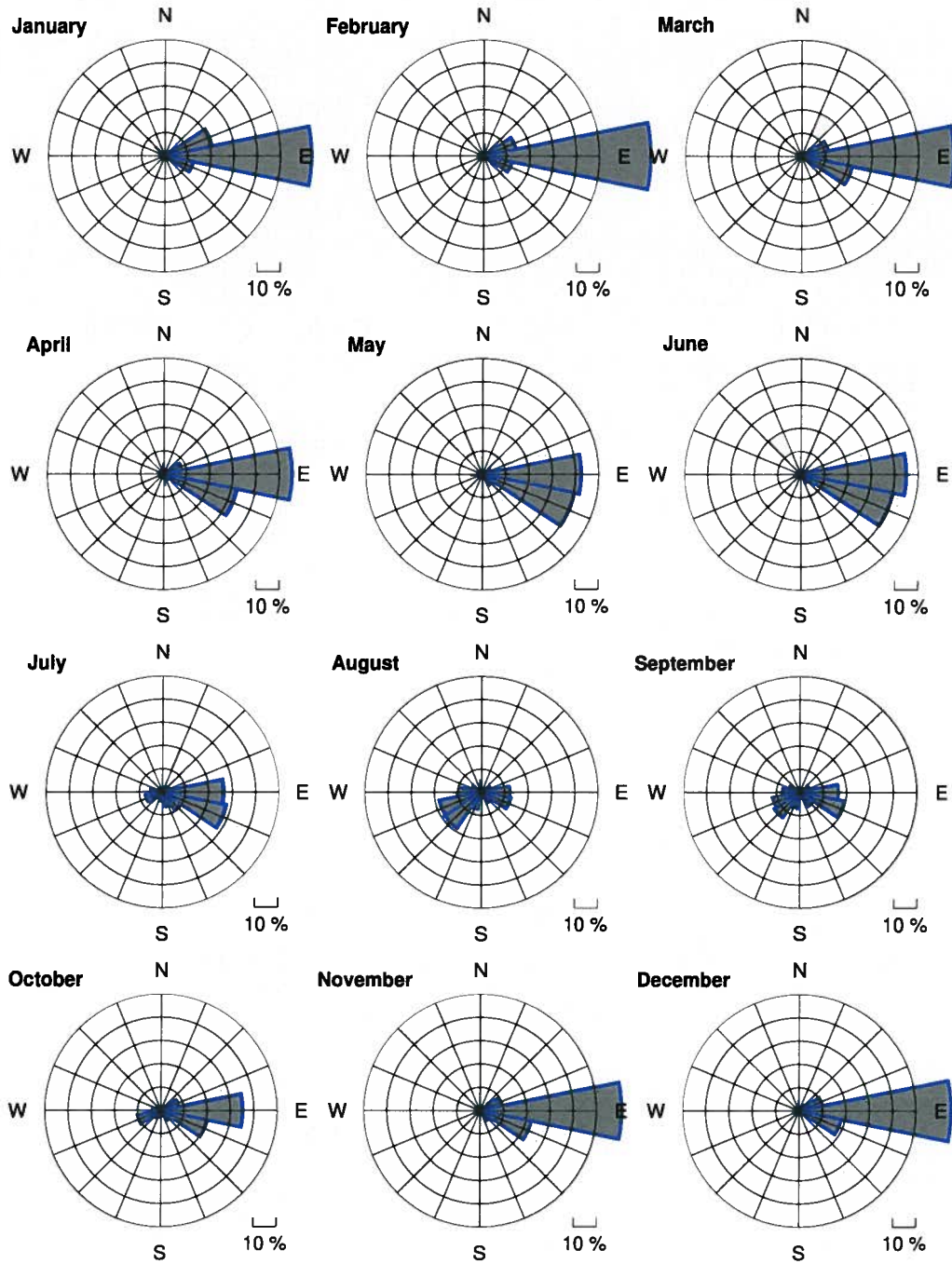
Figure 6: Monthly power roses (for the GEVMP32/275L turbine) for reference point R01
