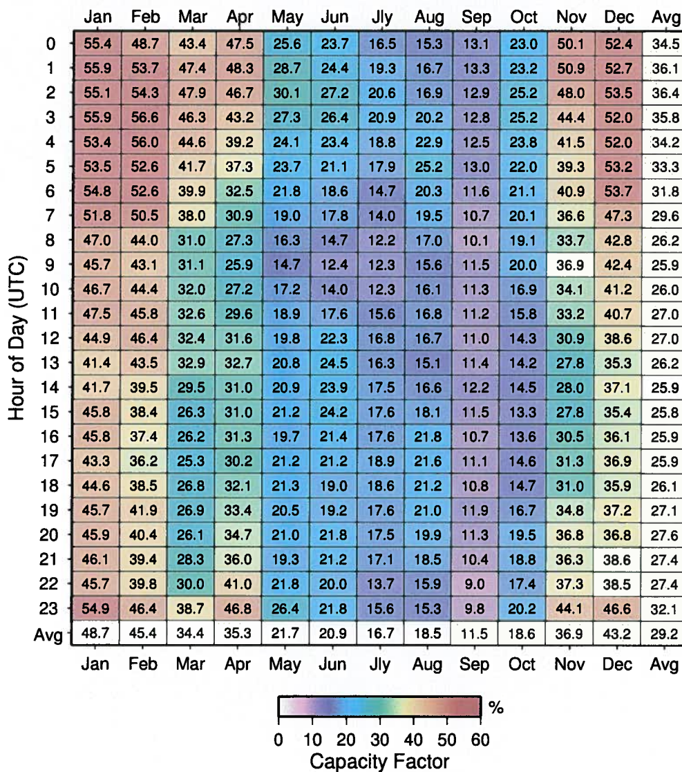
Figure 8: 12 month by 24 hour table of net capacity factor for the GEVMP32/275L turbine. These net values are derived from the gross values using the loss factors in Table 3.
