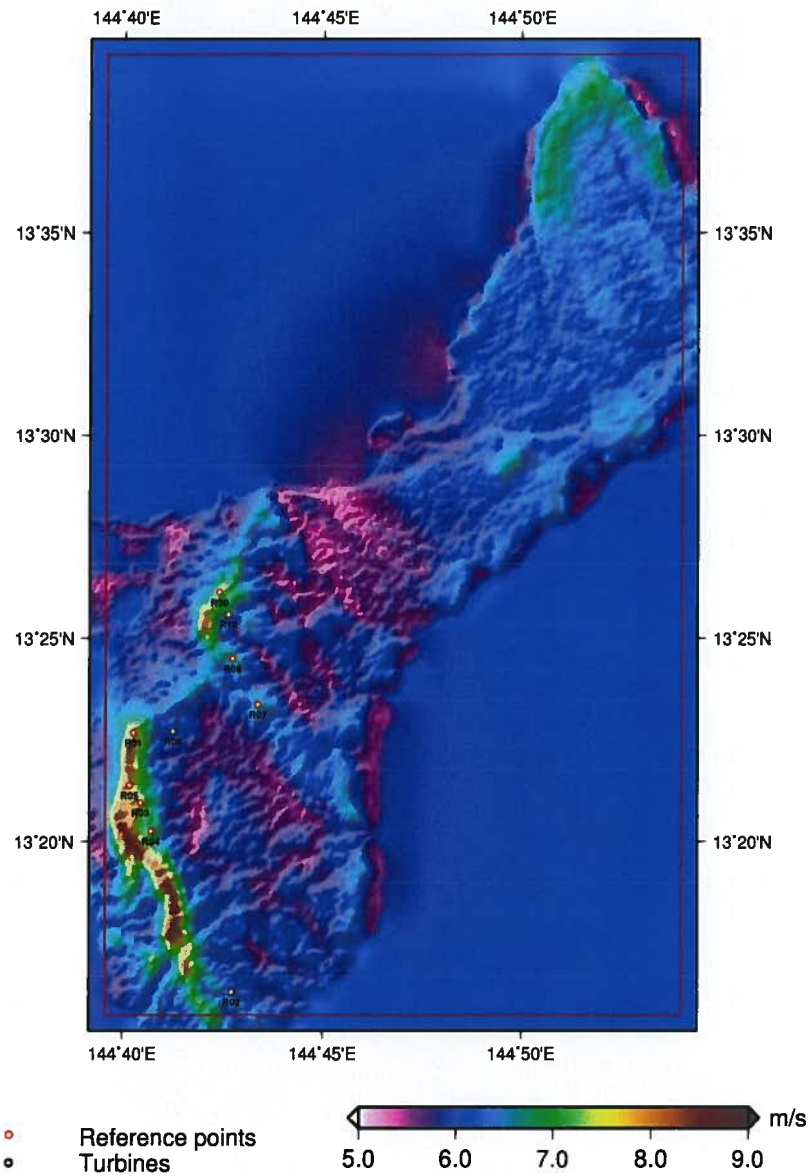
Figure 1: Mean wind speed at 55m.
