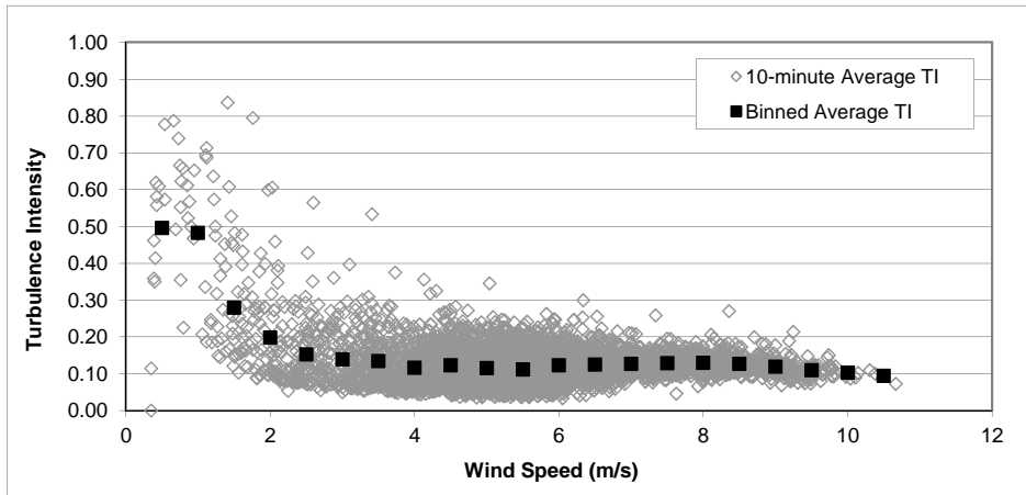
Average Turbulence Intensity by Wind Speed - Site 0001 (60 m)
