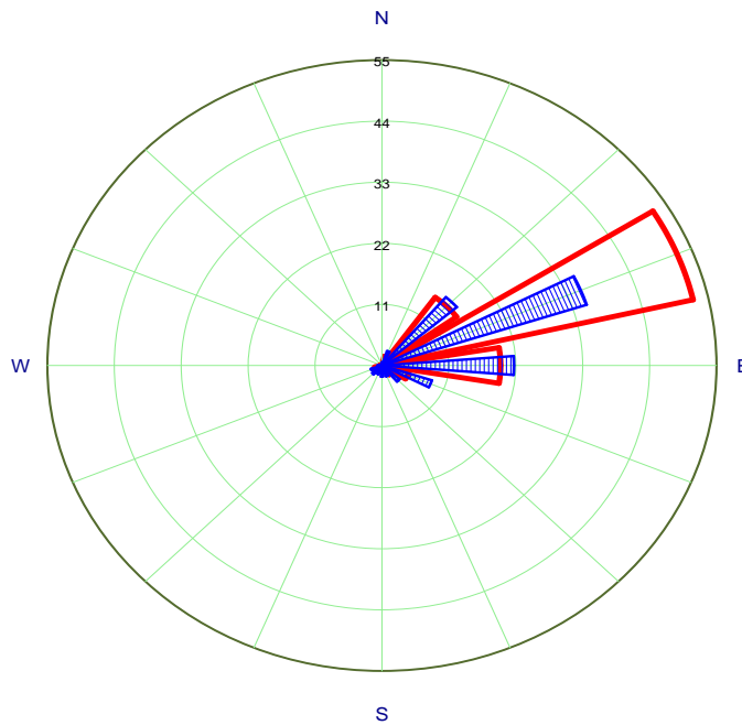
Cumulative Wind Rose (60 m)
