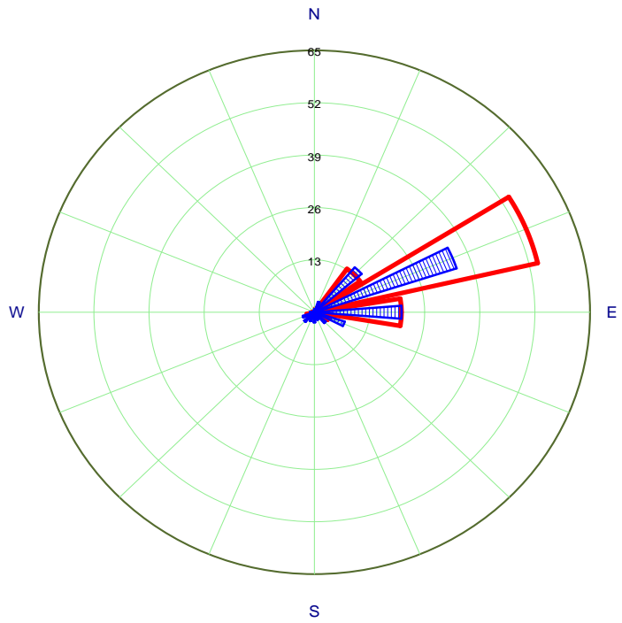
Monthly Wind Rose (60 m)
