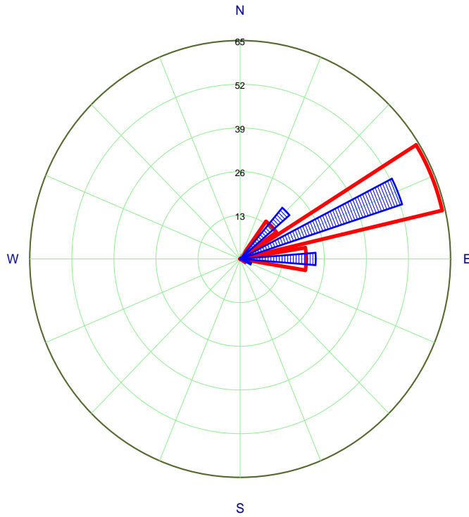
Monthly Wind Rose (60 m)
