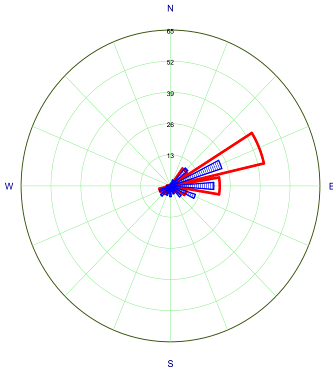
Cumulative Wind Rose (60 m)
