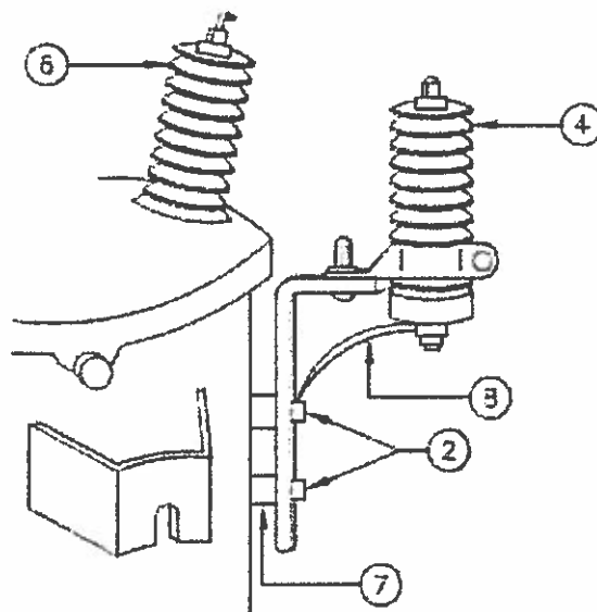
BRACKET MOUNTING DETAIL
