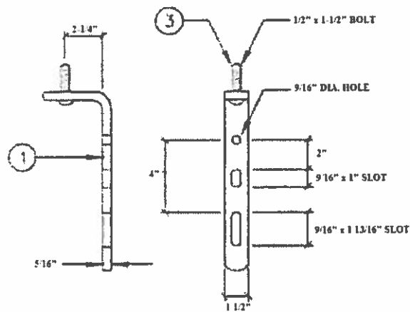
BRACKET DETAIL
