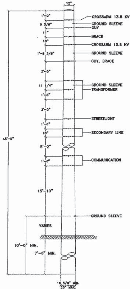
45 FOOT CONCRETE POLE (CLASS B GUYED)
