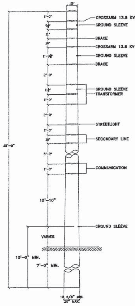
45 FOOT CONCRETE POLE (CLASS A SELF-SUPPORTING)
