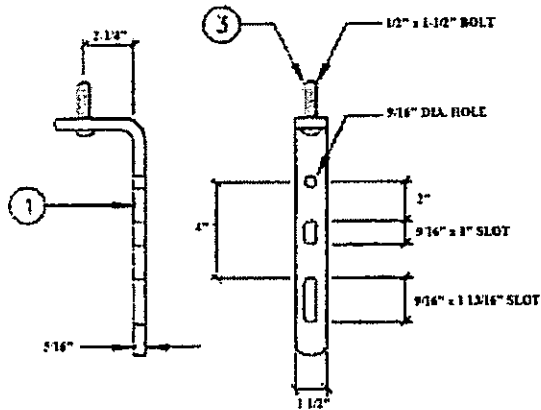
BRACKET DETAIL
