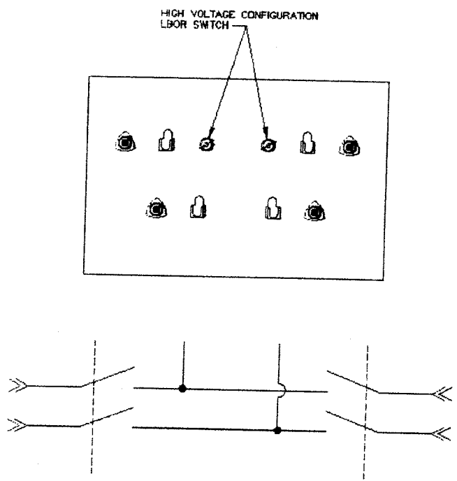
Loop Feed, Dead Front With LBOR Switching
