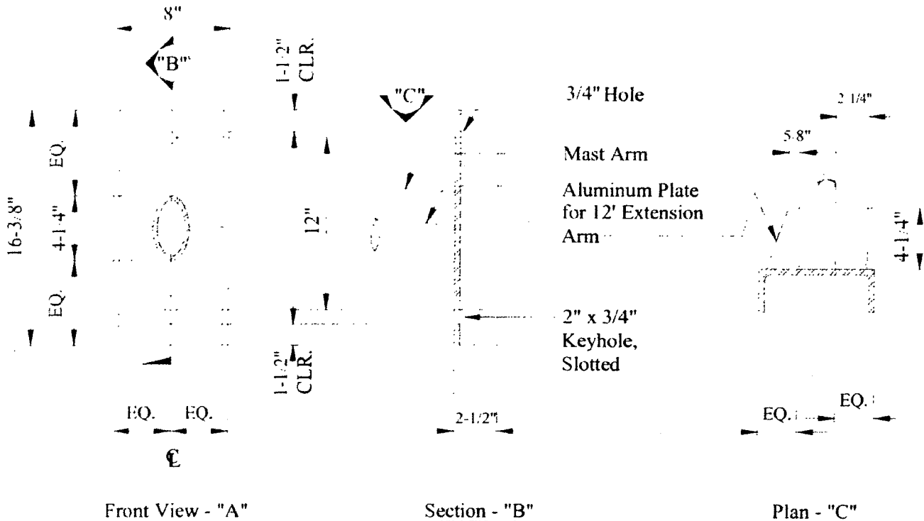
Mounting Plate Detail Figure 2
